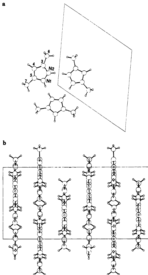
Figure 2. X-ray structure of 3,5-dimethylpyrazole (I): (a) a view of the cyclic trimer projected along the c axis and (b) a molecular packing view projected along the b axis 37 showing the planarity of the trimer.
